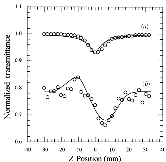
Fig. 4 The Z-scan data of [\text{NEt}_4][\text{PdW}_2\text{S}_8] 2 in acetonitrile, concentration 1.6 \times 10^{-3} \text{ mol dm}^{-3} , at 532 nm with incident energy of 140 \mu\text{J} per pulse, \alpha_0 = 99 \text{ m}^{-1} : (a) collected in the open-aperture configuration and showing NLO absorption [solid curve is a theoretical fit based on equations (1) and (2)]; (b) the Z-scan data and curve (displaced downward by 0.2 from 1.0 for clarity) obtained as in Fig. 3
